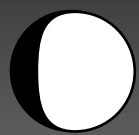
Waxing Gibbous
